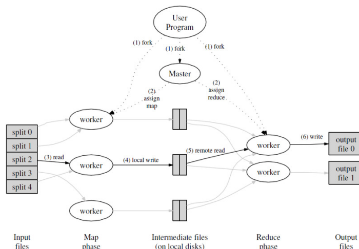
Fig. 2 Execution Overview of MapReduce
