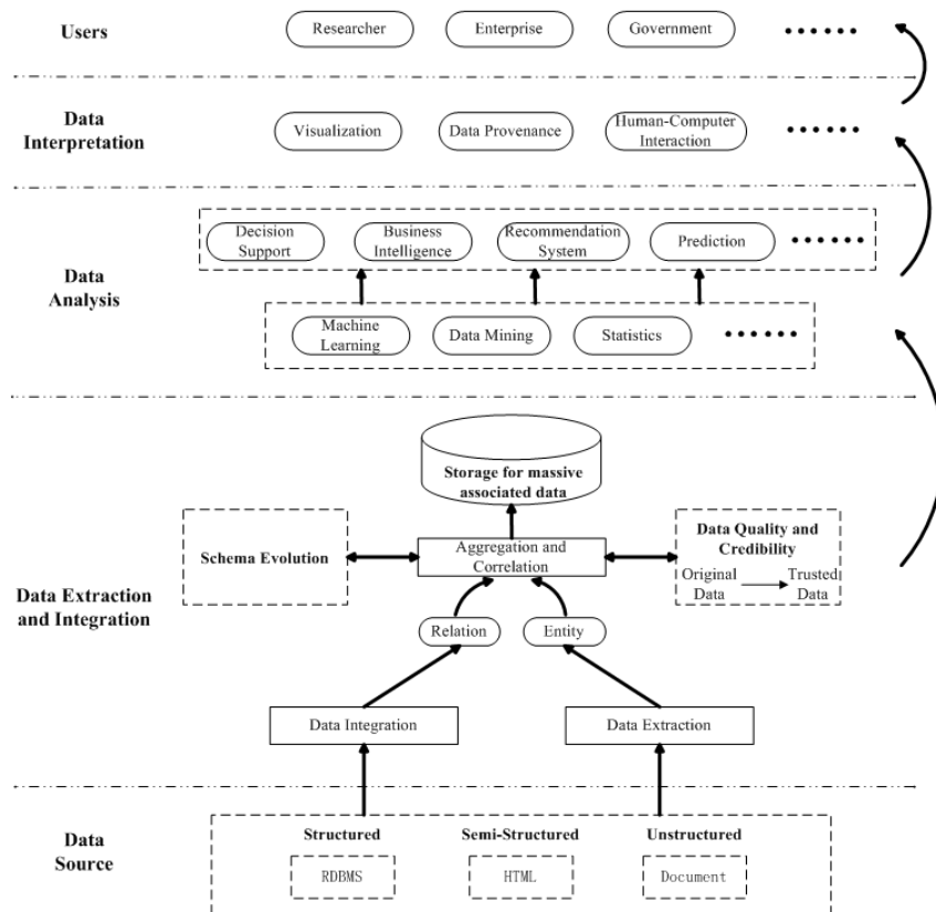
Fig. 3 Basic Framework of Big Data Processing
