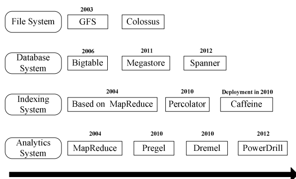
Fig. 4 Technology Evolution in Google
