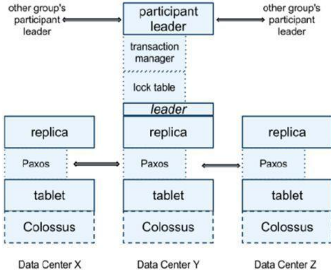
Figure 2: Spanserver software stack.
